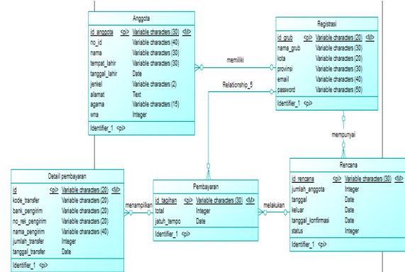
Gambar 4. Conceptual Data Model
