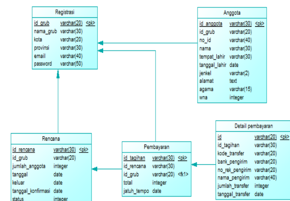
Gambar 5. Physical Data Model
